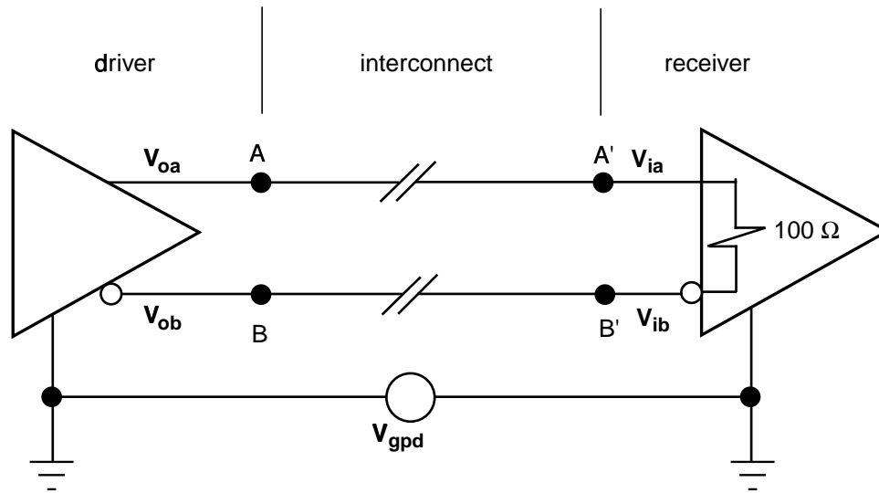
Figure 3–1: LVDS interface
