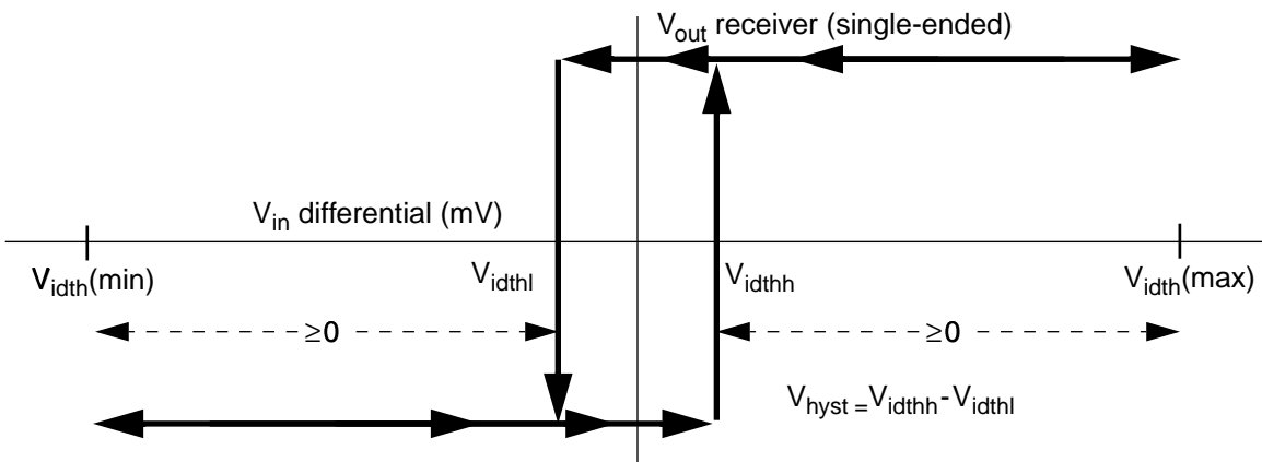
Figure 3-17: Receiver hysteresis
